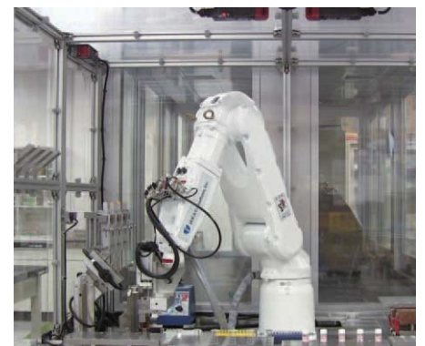
Pre-treatment robots for PCB analysis
