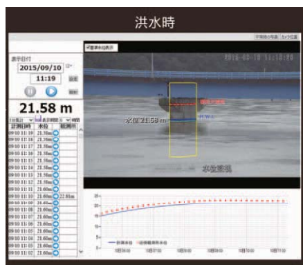
River water level measurement system using CCTV
